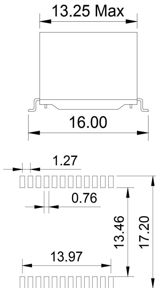
SUGGESTED PAD LAYOUT
