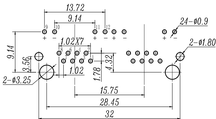
PC Board Layout Top View
