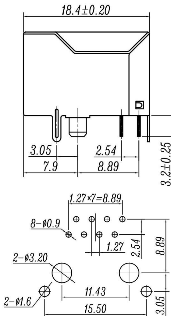
PC Board Layout Top View
