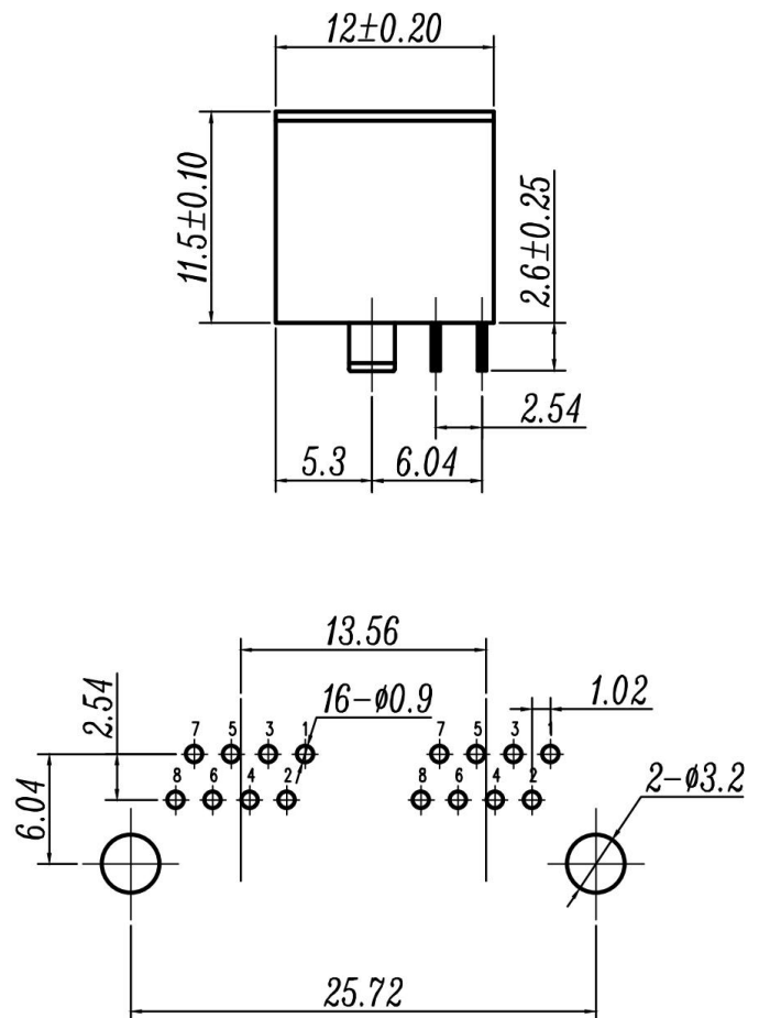
PC Board Layout Top View
