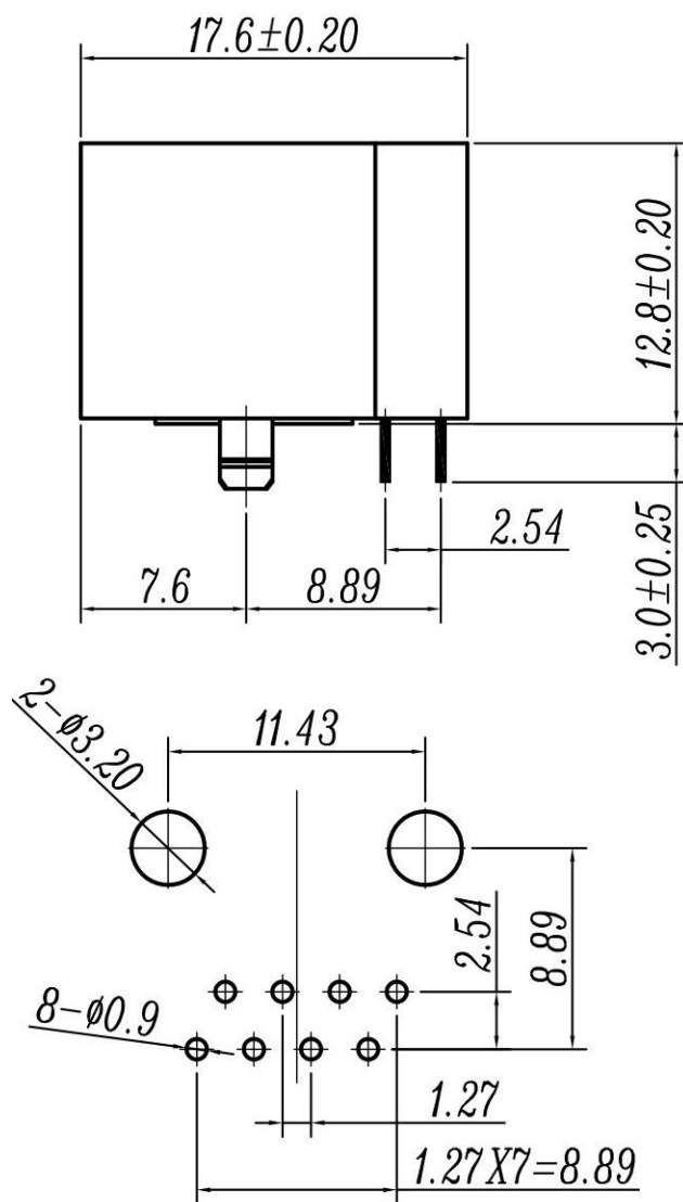
PC Board Layout Top View
