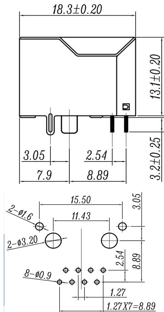
PC Board Layout Top View
