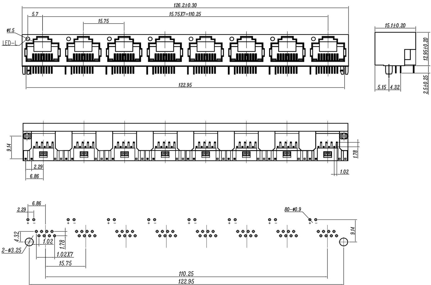
PC Board Layout Top View
