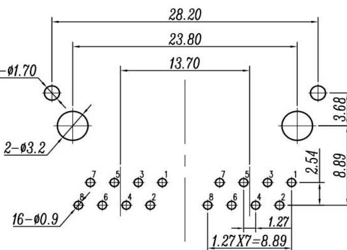
PC Board Layout Top View
