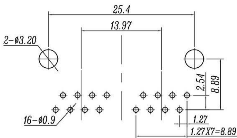
PC Board Layout Top View
