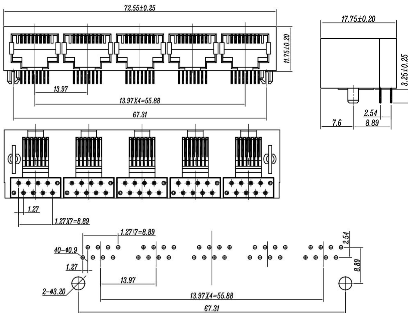
PC Board Layout Top View
