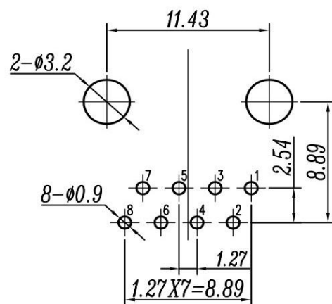
PC Board Layout Top View
