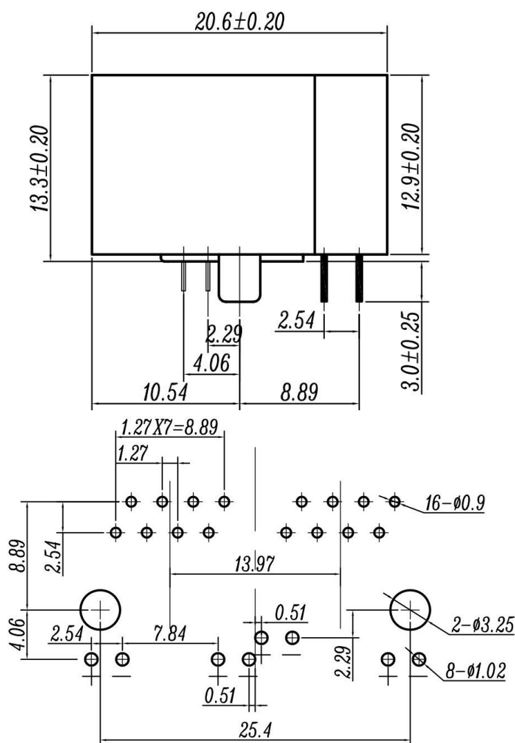
PC Board Layout Top View
