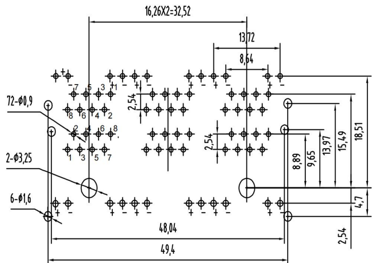
PC Board Layout Component Side Shown
