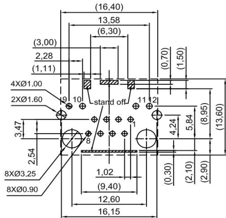
Recommend PCB Layout( Top View) All dimension Tolerance:±0.05
