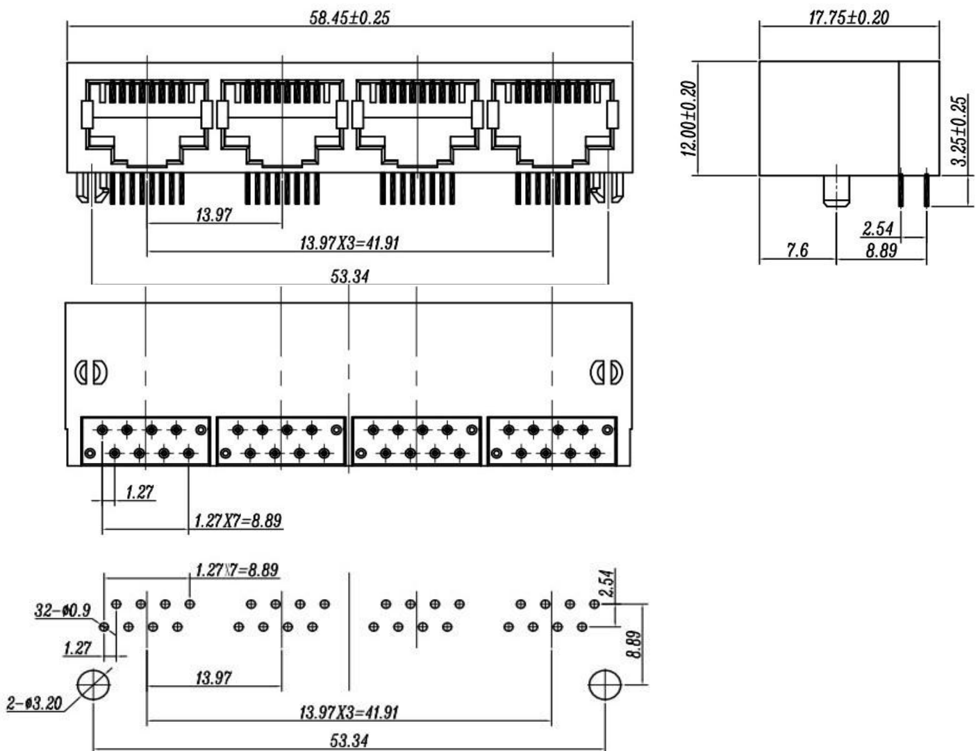
PC Board Layout Top View
