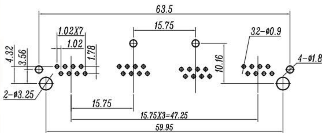
PC Board Layout Top View
