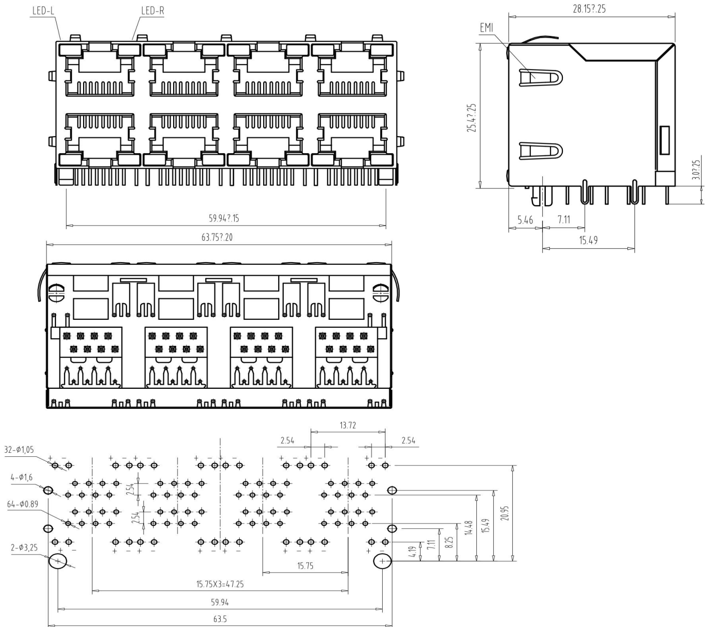
PC Board Layout Component Side Shown
