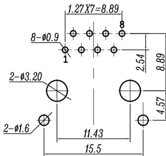
PC Board Layout Top View
