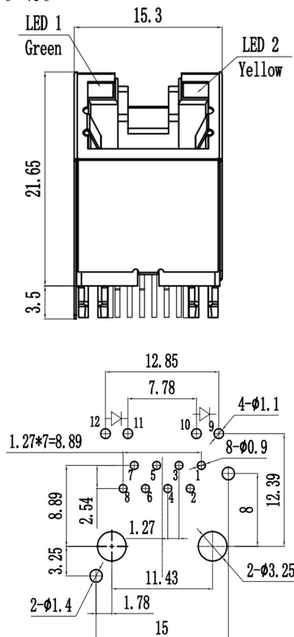
PC Board Layout Component Side Shown
