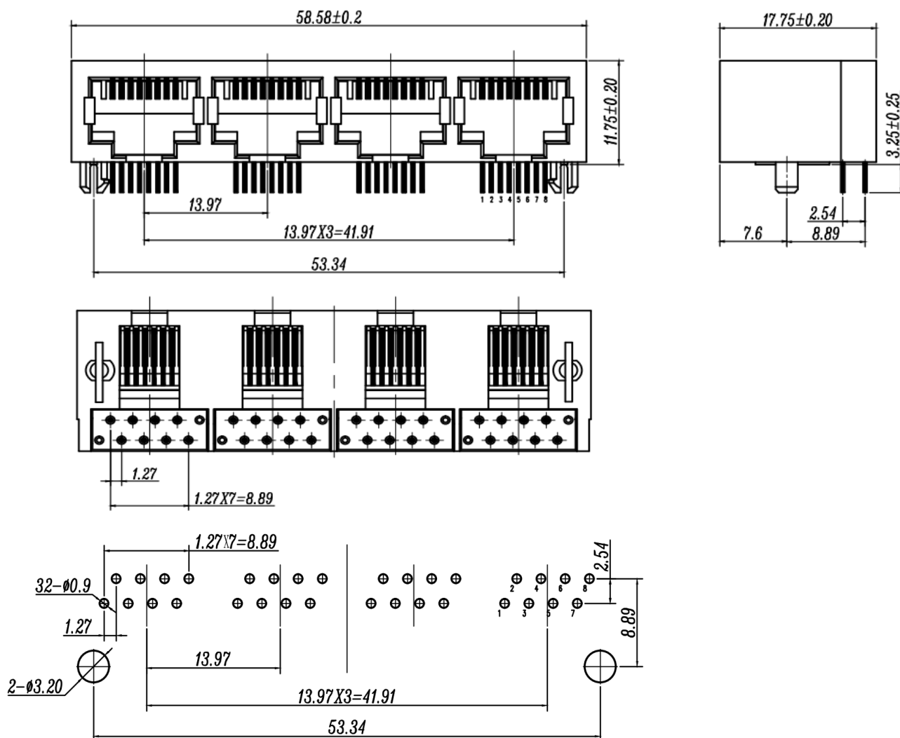
PC Board Layout Top View
