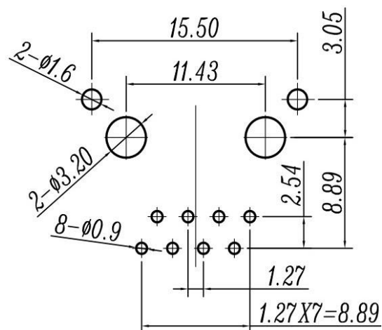
PC Board Layout Top View
