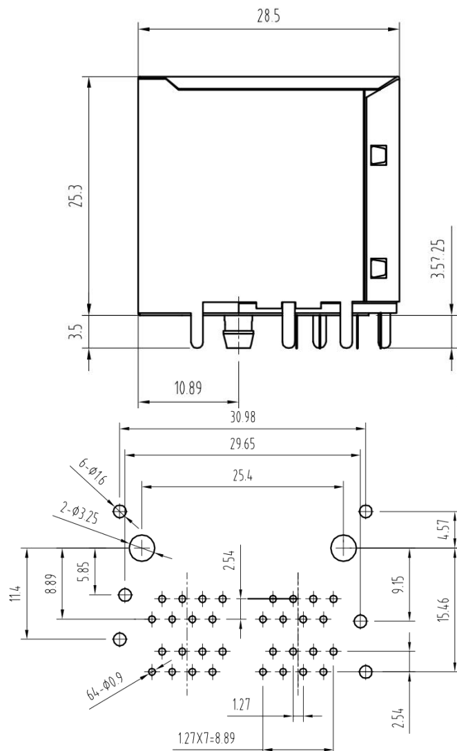
PC Board Layout Component Side Shown
